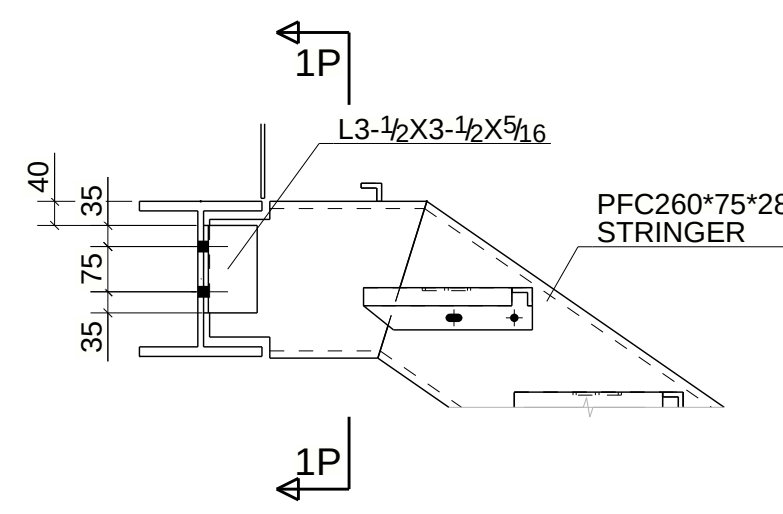
DETAIL - 9
