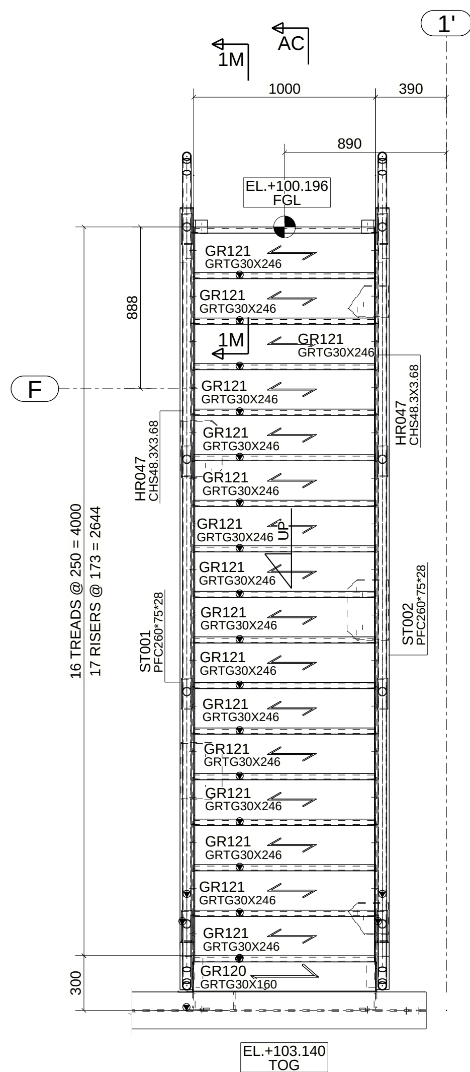
STAIR FRAMING PLAN
