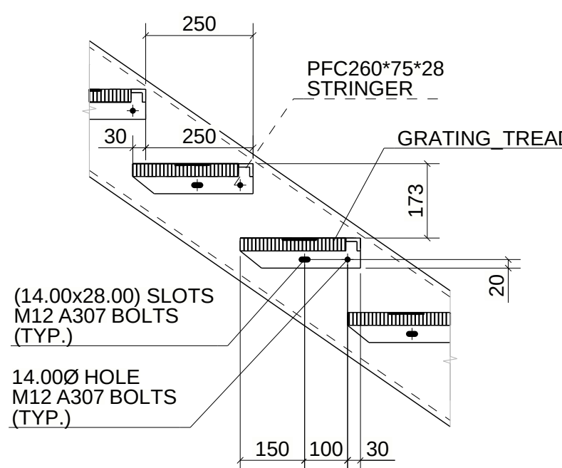
TYPICAL TREAD DETAIL
