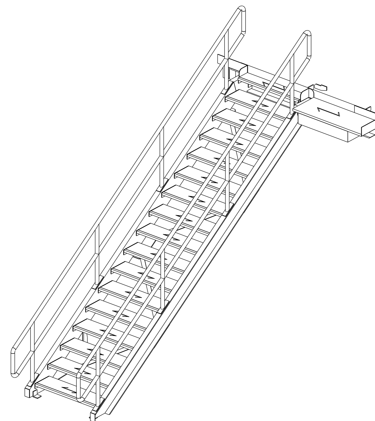
STAIR 3D-VIEW
