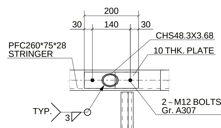
POST CONNECTION TO STRINGER
